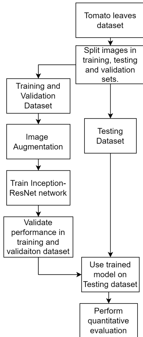
Figure 2: Flow chart for the Inception-Resnet network-based classification
